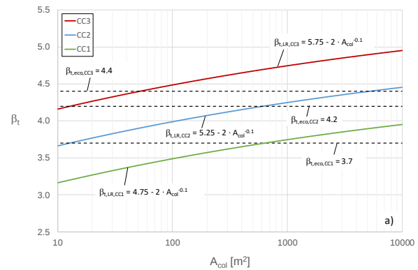
Figure 1. Annual reliability requirements for human safety, \beta_{t,LR} , depending on the collapse area, A_{col} , and the consequence class, CC [2], recommended for the design of key members; \beta_{t,eco} [17]: tentative target reliabilities based on economic optimisation for medium relative cost of safety measures and different consequence classes, CC.
