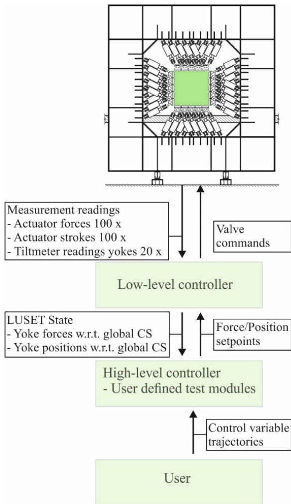
Figure 4. LUSET control software architecture; adopted from [1].
