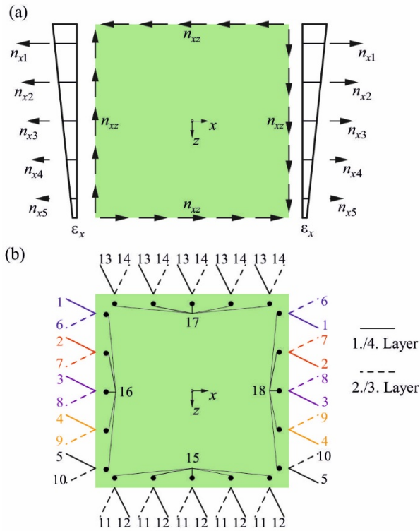
Figure 6. Non-homogeneous panel test in the LUSET, with shear loading and imposed longitudinal strain with a gradient: (a) loading; (b) machine configuration; adopted from [1].
